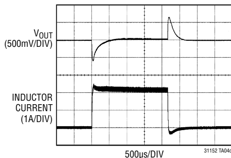
0A to 1.5A Load Step, V IN = 10.6V
