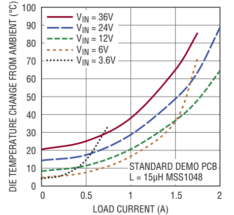
Die Temperature Rise vs Load Current, V_{OUT} = 5V , f_{SW} = 1.5MHz
